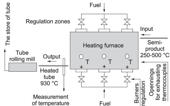
Figure 1 Heating furnace...
